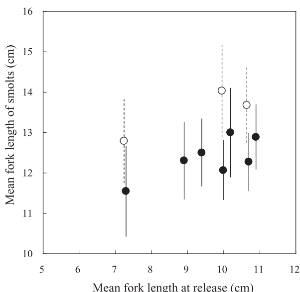
Fig. 30 Mean fork length of hatchery-origin 1+ (○) and 2+ (●) masu salmon smolts captured at the upper partial fence in the Masuhoro River, 1995-1999, in relation to the mean fork length at release in the preceding fall. Error bar indicates standard deviation.
