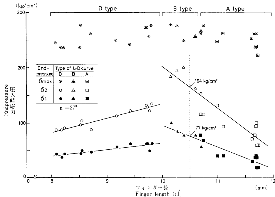
第16図 嵌合縦圧縮試験におけるフィンガー長と圧入時応力の関係 Fig. 16 Relationship between endpressure and (finger length for inserting test. Footnote *: Data of specimen No. 14, 22, 25, 28, 31 are excluded from the figure.
